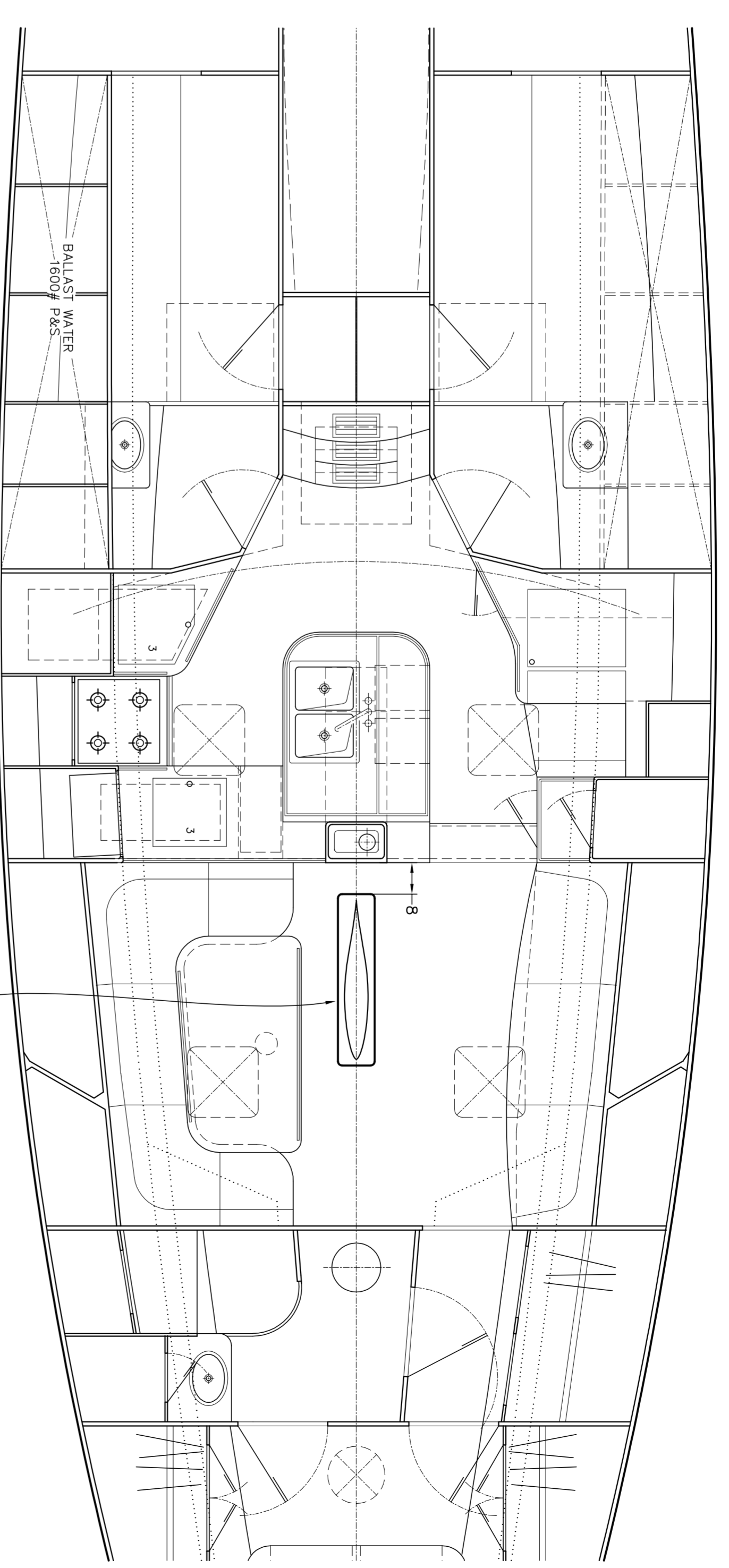
PLAN SALON WITH KEEL TRUNK SCALE 1:25
